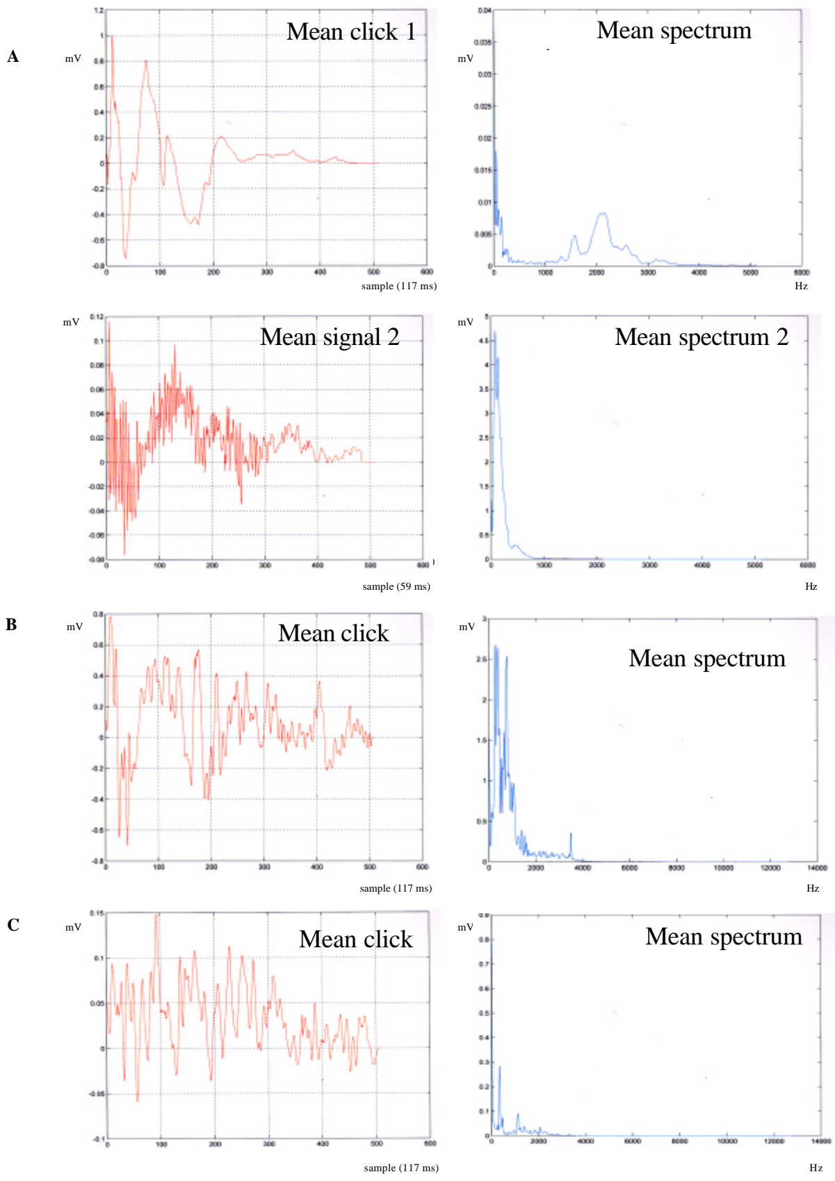
Fig. 1 - signal's mean waveform and mean spectrum of sperm whale (A), long finned pilot whale (B) and Risso's dolphin (C)
