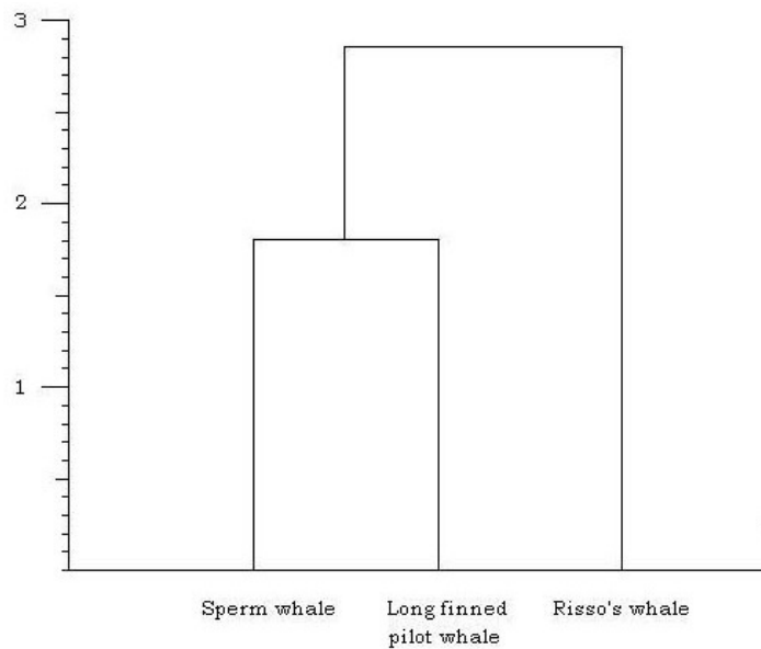
Fig. 2 - dendrogram; the sperm whale ( Physeter macrocephalus ) and the long finned pilot whale ( Globicephala melas ) have acoustic signals more similar between them than the Risso's dolphin ( Grampus griseus ) due to the considerable size of both these two species.
